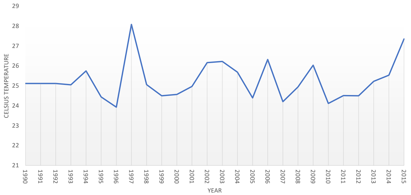
Mean SST - Eastern Equatorial Pacific
